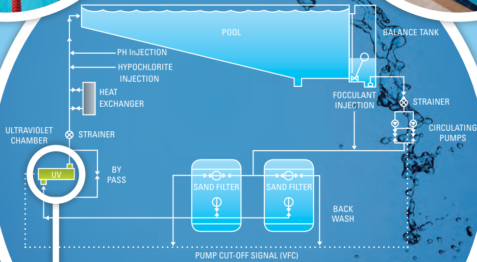
Flow Diagram for Single Pool with Ultraviolet Disinfection
