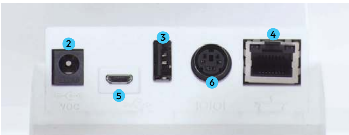
Back view of Microlab 600 Controller
