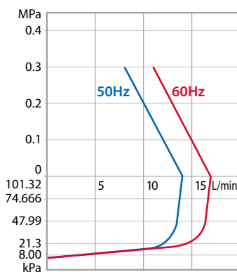
MDG-R15T220
