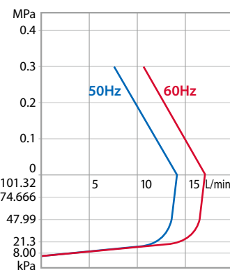
MDG-R15P220
