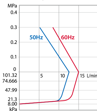
MDG-R15K220, R15C220
